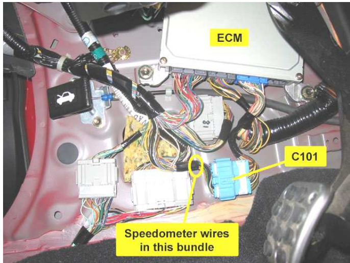
Photo 9 – Attach crimp connectors to speedometer wires as shown
