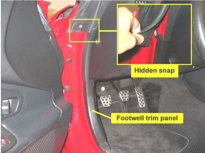
Photo 3 – Remove hidden snap on foot well trim panel
