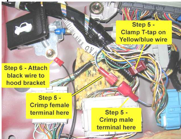
Photo 9 – Attach crimp connectors to speedometer wires as shown
