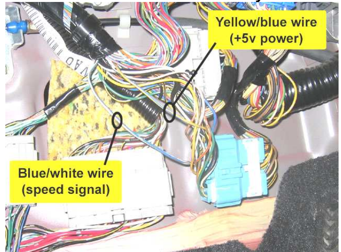
Photo 10 – Attach crimp terminals to Yellow Jacket wire harness as shown
