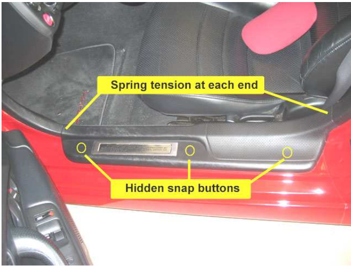
Photo 1 – Remove driver’s door sill trim
